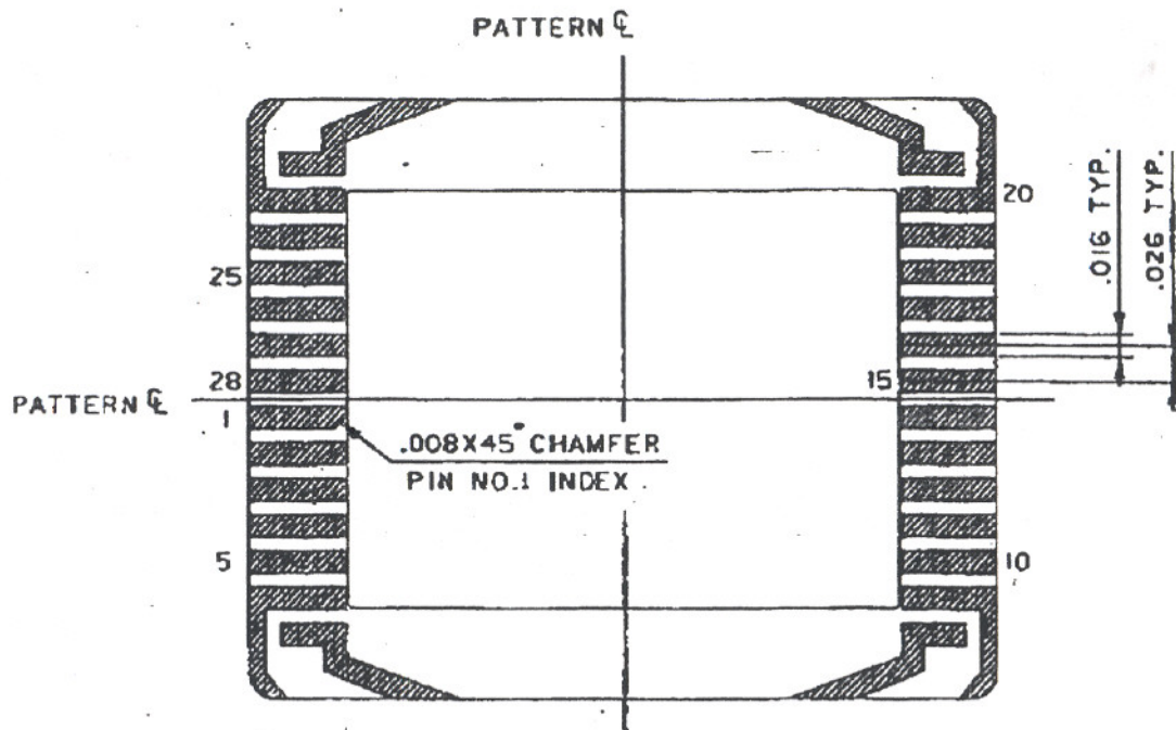
BONDING PATTERN
