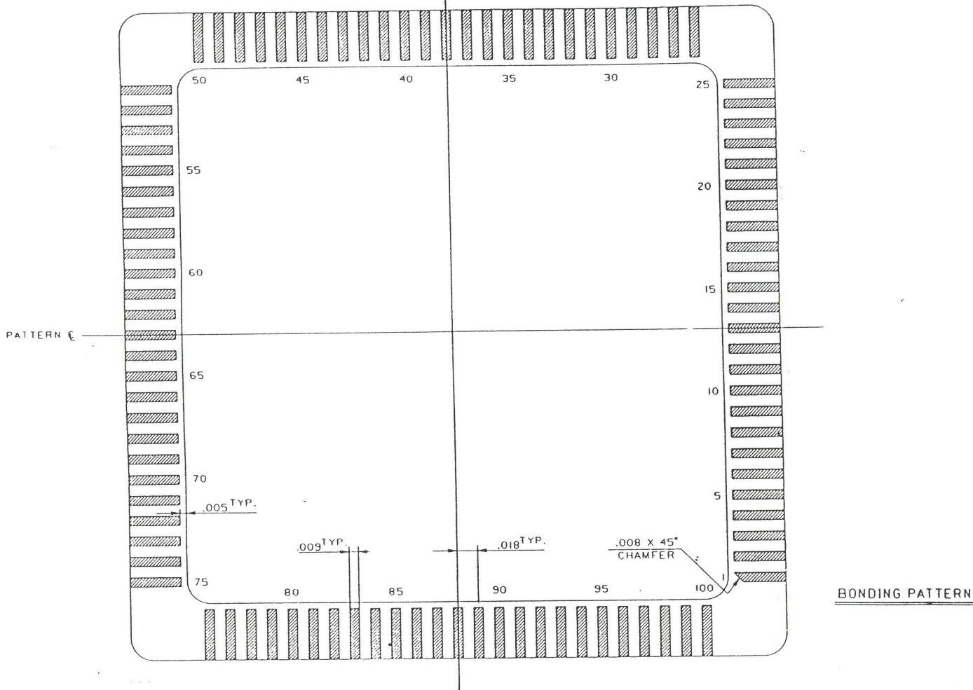
WIRE BOND PAD / CONNECTOR PIN INTERCONNECTION PLAN
