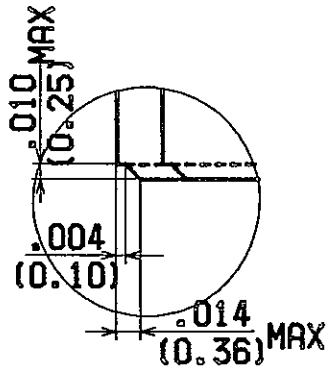
VIEW "P"
